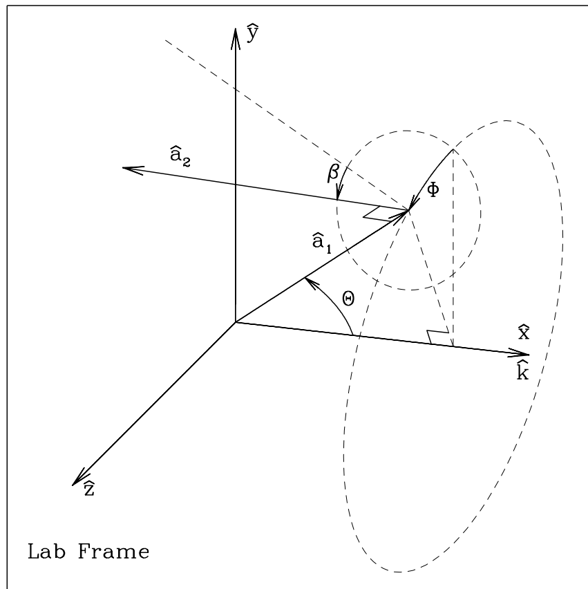
Figure 7: Target orientation in the Lab Frame. \hat{x} = \hat{x}_{\text{LF}} is the direction of propagation of the incident radiation, and \hat{y} = \hat{y}_{\text{LF}} is the direction of the real component (at x_{\text{LF}} = 0, t = 0 ) of the first incident polarization mode. In this coordinate system, the orientation of target axis \hat{a}_1 is specified by angles \Theta and \Phi . With target axis \hat{a}_1 fixed, the orientation of target axis \hat{a}_2 is then determined by angle \beta specifying rotation of the target around \hat{a}_1 . When \beta = 0 , \hat{a}_2 lies in the \hat{a}_1, \hat{x}_{\text{LF}} plane.
